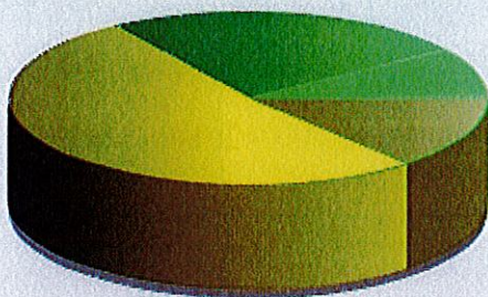
Outgoing vehicles
