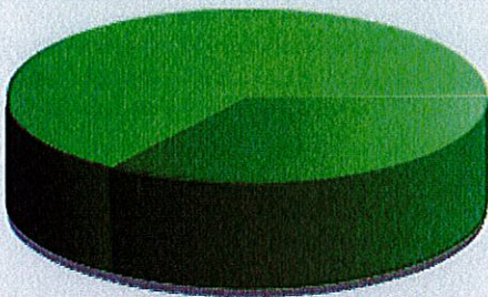
Outgoing vehicles
