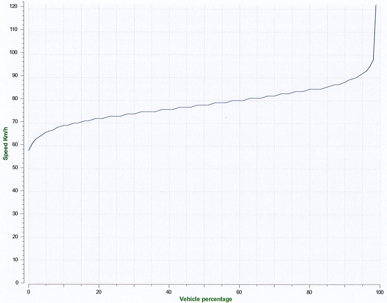
Speed percentile(outgoing)
