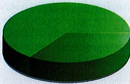
Incoming vehicles
